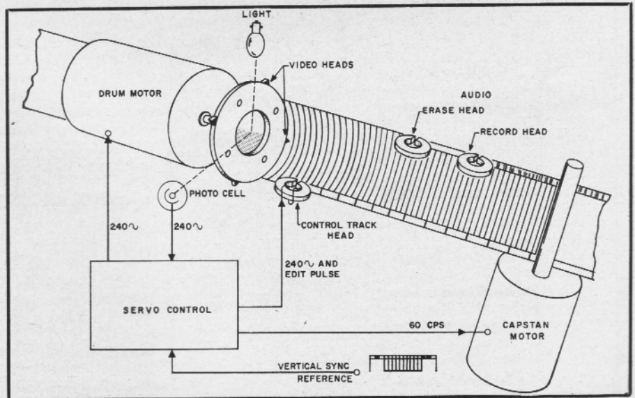
Fig. 3. Simplified diagram showing "Videotape Recorder" in the "record" mode.
