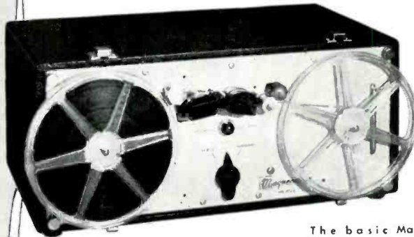
The basic Magne recorder mechanism (PT6-A)
