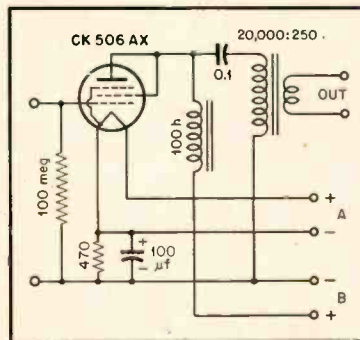
Fig. 7. Single-stage preamplifier schematic.
