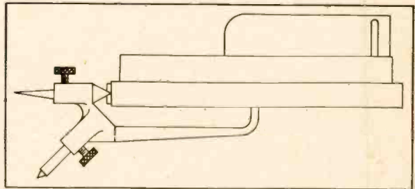
Fig. 1. Early form of acoustic reproducer employing two needles for reproduction of both lateral and vertical (hill and dale) discs.
