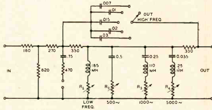
Fig. 3. Circuit of crossover filter.
