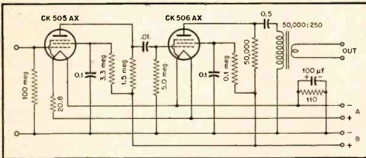
Fig. 4. Basic two-stage preamplifier.
