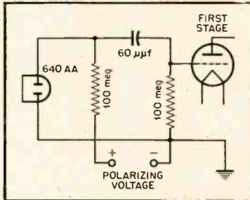
Fig. 3. Input circuit of preamplifier.
