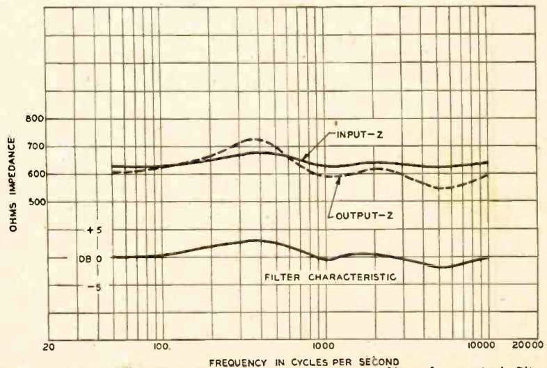
Fig. 4. Input and output impedance of crossover filter for typical filter adjustments.
