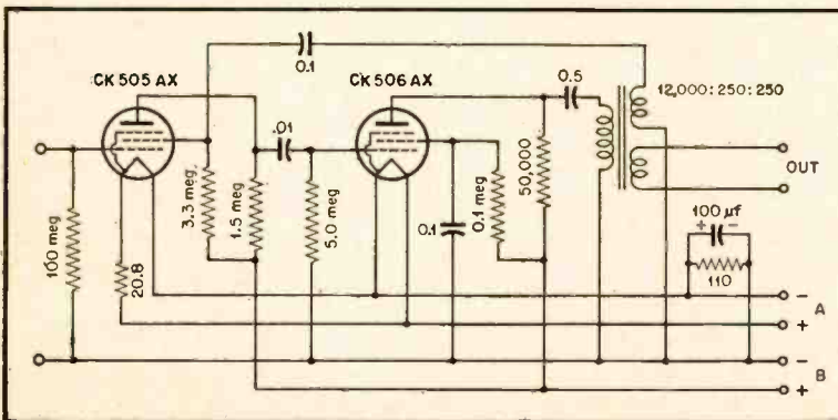
Fig. 5. Two-stage preamplifier with over-all feedback.
