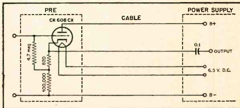
Fig. 9. Cathode-follower preamplifier schematic.
