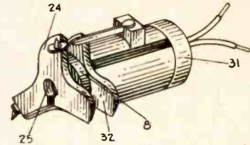
Fig. 4. Polyphase reproducer arranged for mounting of three styli. As shown, upper stylus is for lateral records, one at lower left is for vertical transcriptions.
