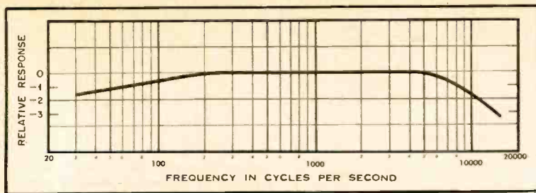
Fig. 6. Frequency response of a two-stage preamplifier with over-all feedback.
