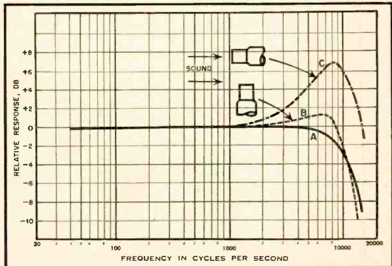
Fig. 1. Response of typical 640AA condenser microphone under various conditions: (A), with constant sound pressure at the diaphragm; (B), in free field with sound passing across the diaphragm; (C), in free field when pointed directly at sound.
