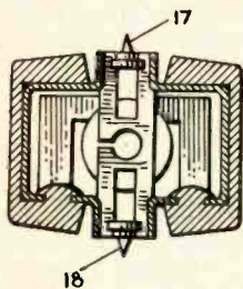
Fig. 2. Drawing of end view of new Polyphase reproducer with two separate styli, single magnet and voice-coil.
