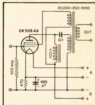
Fig. 8. Single-stage preamplifier with feedback.
