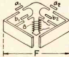
Fig. 3. Equivalent magnetic circuit corresponding to a balanced bridge.
