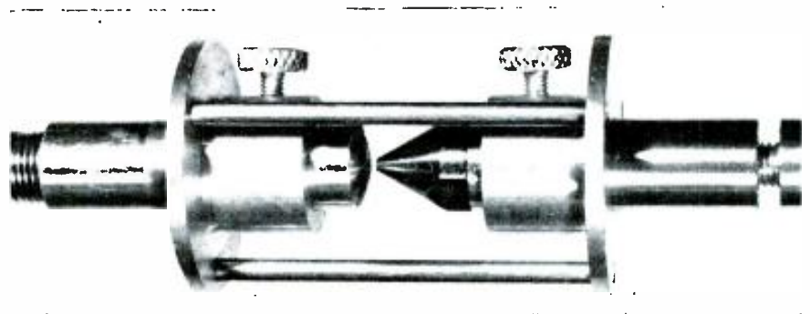
Close-up view of the Hartmann whistle.
