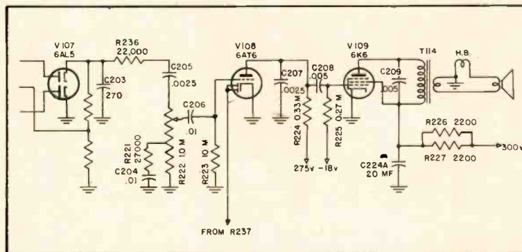
Fig. 1. Audio section schematic of RCA 630TS receiver chassis.
