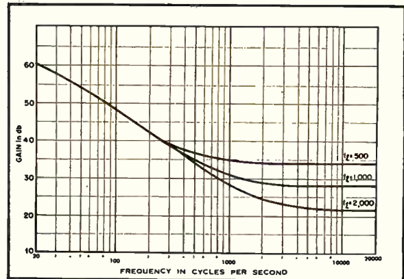
Fig. 6. Response curves obtained with second preamplifier.
