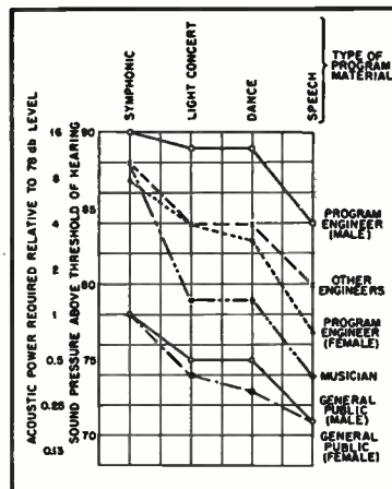
Fig. 1. Preferred average maximum sound pressure levels.
