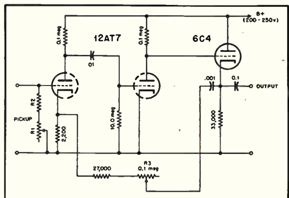
Fig. 5 (right). Schematic of second preamplifier, with continuously variable turnover point.
