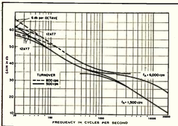
Fig. 4 (left). Typical response curves obtained with first preamplifier.
