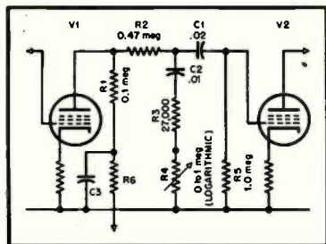
Fig. 6. Interstage bass-compensation circuit.
