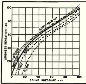
Fig. 3. Relative loudness sensation in the mind for frequencies above 1000 cps.
