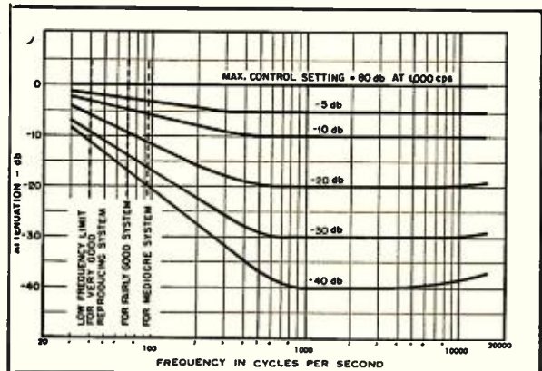
Fig. 4 (left). Over-all transmission characteristic of human hearing system. Fig. 5 (right). Theoretical response of volume control compensated to 80-db standard.
