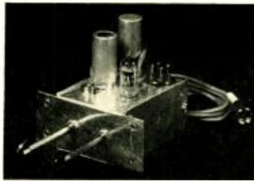
Fig. 7. External view of second preamplifier.
