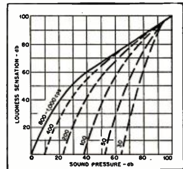
Fig. 2. Relative loudness sensation in the mind for frequencies below 1000 cps. Reference of 0 db corresponds to threshold of hearing, and a 6-db change represents a sound pressure ratio of 2 to 1.
