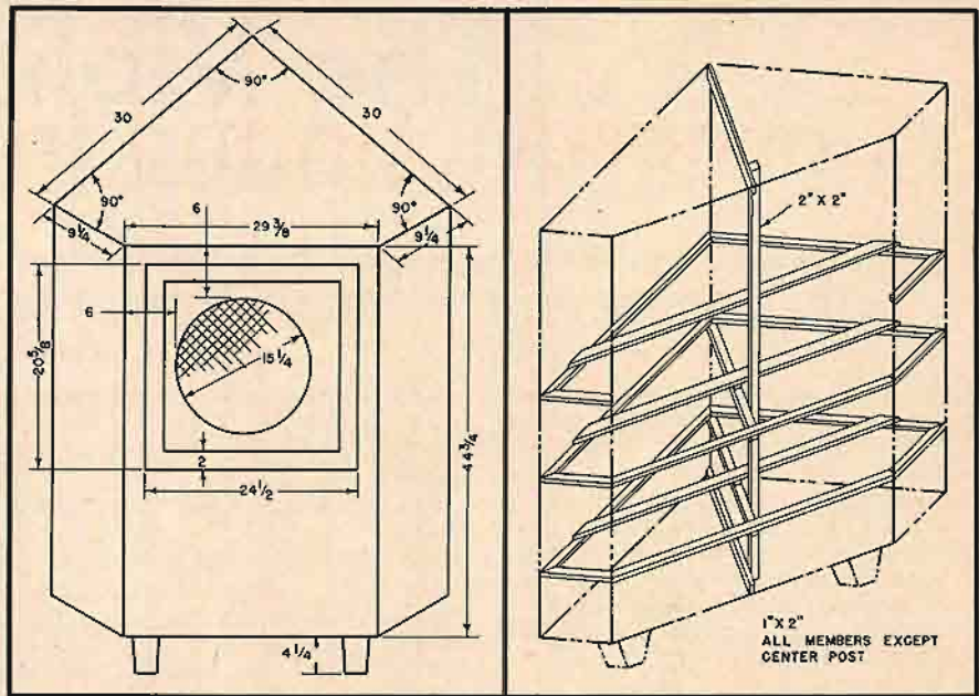
Fig. 2. Constructional details for the corner-mounted infinite baffle.
