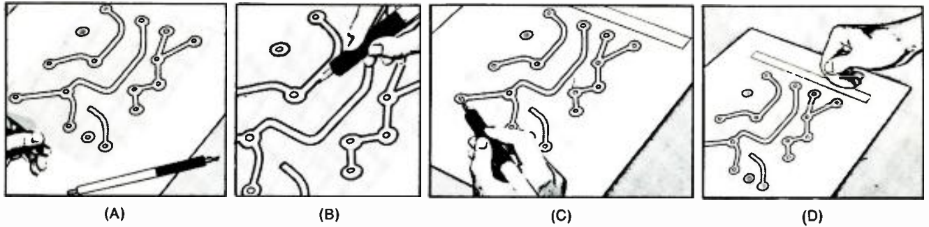
Figure 1. The steps necessary to use Ulano Rubyolith® masking films. In (A) a sheet of this transparent deep red material is placed above the original drawing. A sharp knife traces the circuit paths (B) cutting through the red coating. Then lifting the edge with the knife, (C) the red is stripped off (D) leaving a clear plastic coating underneath. This can then be used as either a positive or negative for the etching procedure.
