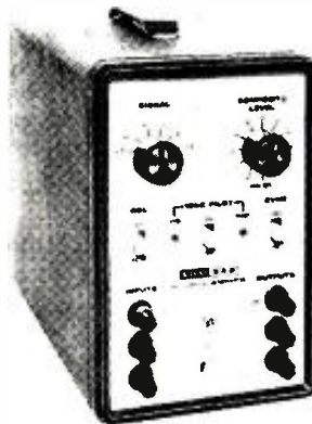
EICO 342 FM Multiplex Signal Generator Crystal-controlled 19 kHz ( \pm 2 Hz) pilot. Both composite audio and f.m. r.f. outputs. F.m. stereo broadcasting from tape. phono/oscillator source. Low distortion signals to permit alignment for lowest distortion. $175.00
