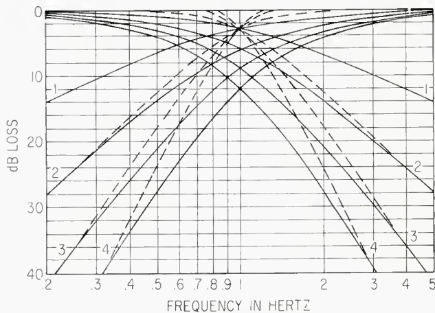
Figure 2. A fallacy of using multi-stage crossovers as frequency dividers that do not possess interaction or active feedback. The solid curves show the result of cascading the shown number of identical roll-off networks, while the dashed line curves show the required response.
