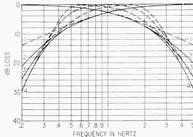
Figure 3. By changing the frequencies of curves for two or more networks, the 3-dB point can be corrected, as shown here (solid curves). But the result does not differ appreciably from a single network, until about an octave beyond crossover. The dashed line curves show the true responses similarly frequency-shifted.
