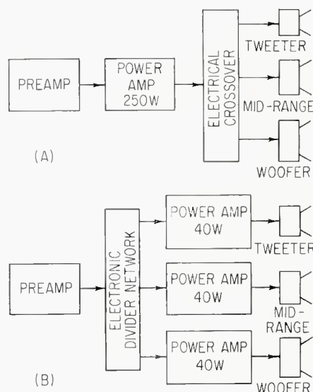
Figure 1. The choice between systems using crossover frequencies: (A) the conventional electrical system, where the crossover divides frequency distribution after power amplification, as energy is fed to the speaker units; (B) electronic frequency division, before power amplification.
