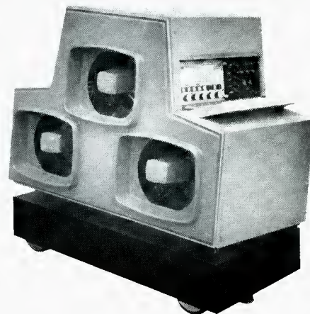
Figure 1. Amphicon's three-section large-screen color projector, model Amphicolor 1000. Note the easily-accessible controls.
