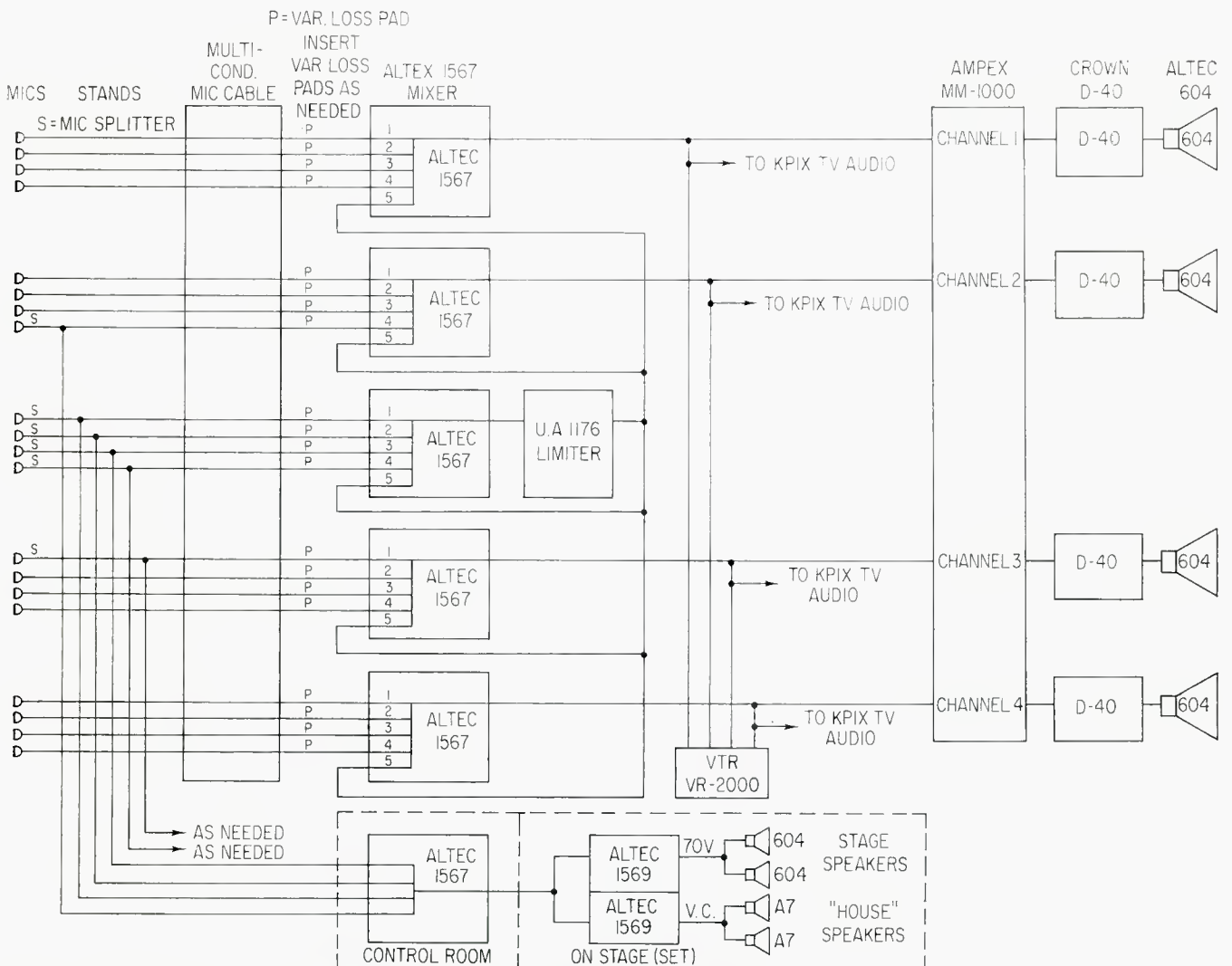
Figure 2. This is the way the audio signals went to get to the correct stations in the correct way.
