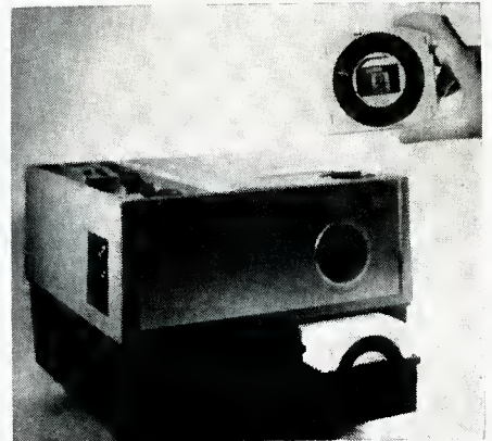
Figure. 2 The 3M sound-slide projector. It uses a standard 2 x 2 slide ringed by the sound track.
