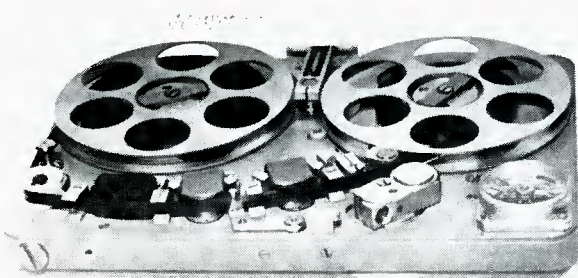
Figure 2. The new Nagra SN miniature tape recorder.
