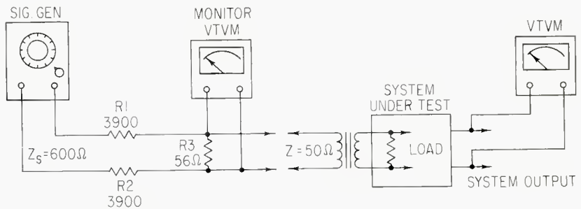
Figure 1. A balanced resistive pad for low-impedance, low-level loads.
