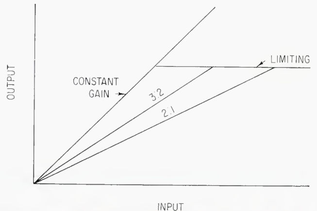
Figure 1. Idealized graphs of compressor and limiter functions.
