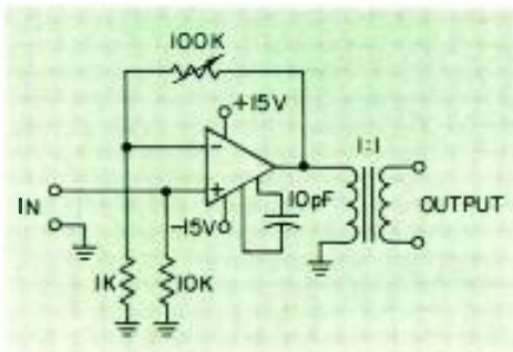
Figure 1. An integrated circuit as a line amp without a current booster.
