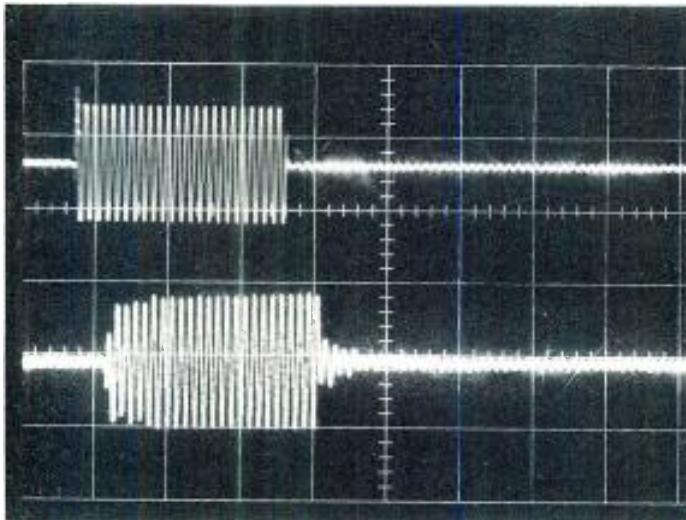
Typical toneburst response of a medium quality domestic loudspeaker system. Upper trace: amplifier input; lower trace: loudspeaker output.
