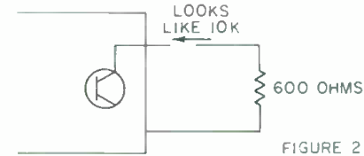
Figure 2. Connecting an output load to amplifier can change things, with or without feedback.
