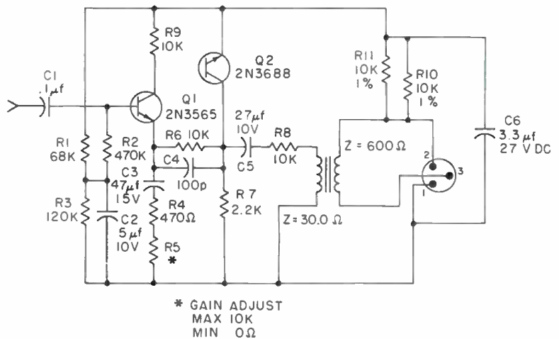
Designed for Leon Russell House Studio, above circuit is for a direct box that is phantom-powered from an API console.
