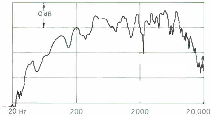
Axial frequency response of a well-known studio monitor system.
