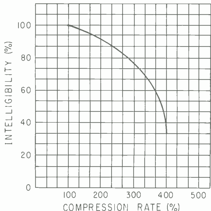
Figure 2. Speech intelligibility vs. compression rate curve (after Garvey).
