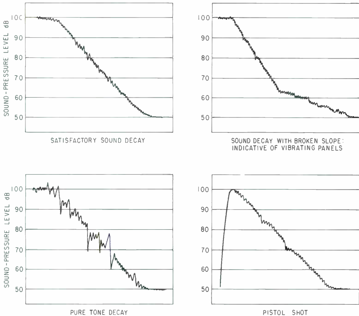
Figure 2. Sound decay curves recorded in various studios.
