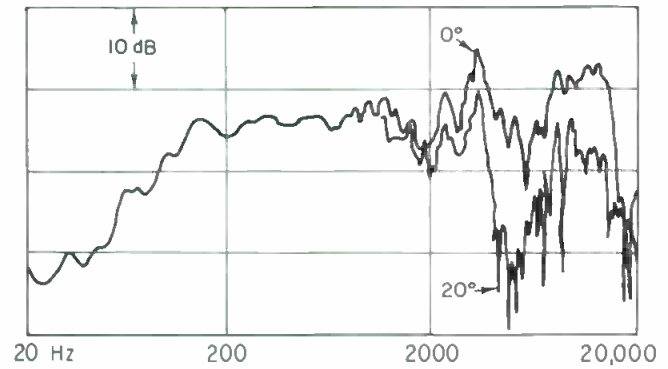
Axial and off-axis (20 degrees) response of an inexpensive ($15) domestic speaker in a 0.3 cu. ft. cabinet.
