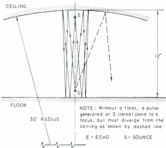
Figure 1. Geometric construction of echo produced by a reflective dome whose radius of curvature is 2.5 times the distance between floor and ceiling. Only the central reflecting area of the dome can produce a sound concentration.
