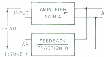
Figure 1. The accepted block diagram for illustrating the action of feedback.
