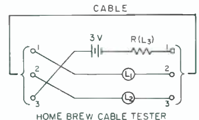
HOME BREW CABLE TESTER
