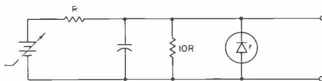
Figure 1. The electrical analog of a sensory receptor membrane.
