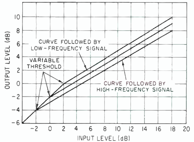
Figure 3. The compression characteristic of a de-esser indicates threshold sensitivity as related to various frequencies.
