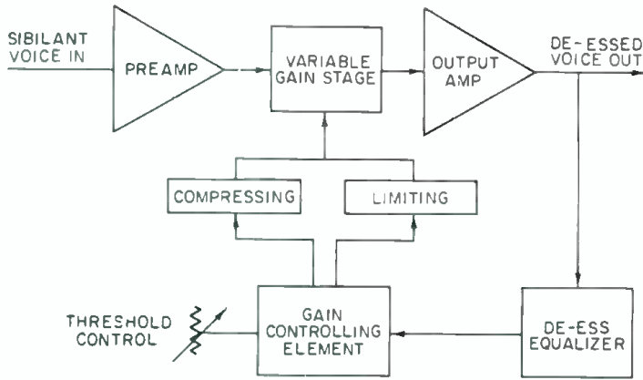
Figure 2. A simplified block diagram of a de-esser system using control-path equalization.
