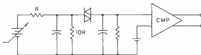
Figure 2. The electrical analog of a sensory-neural junction.
