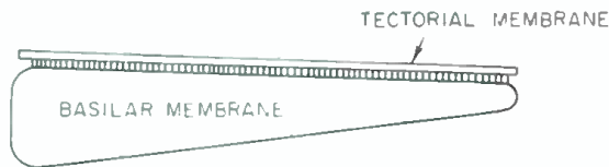
Figure 4. A schematic representation of the hearing receptor mechanism. Relative motion between the basilar membrane (which is excited) and the tectorial membrane produces stress on the hair cells (the sensor-neural transducers).
