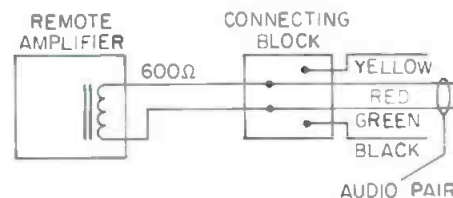
Figure 4. Troubles will develop at the remote site unless the remote amplifier is properly connected to the line. Use only the balanced output of the amplifier and connect it to the red and green wires in the Telco line.
