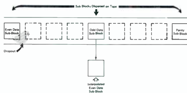
Figure 5. Error concealment by interpolating between samples in a data sub-block.
