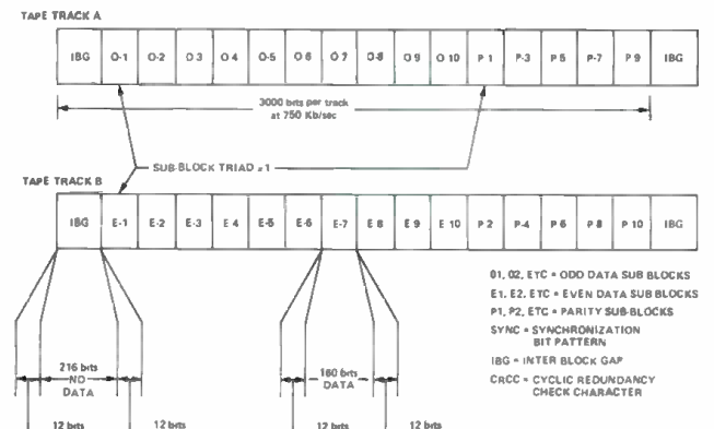
Figure 2. A tape track format.
