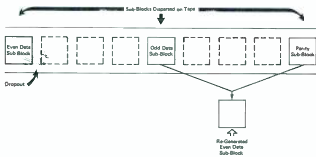
Figure 4. Error correction, using data and parity sub-blocks.
