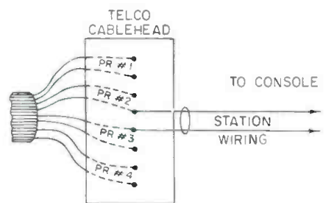
Figure 3. Splitting pairs can cause many problems. Shown here is what is meant by the term. A station audio pair has been connected to two entirely different Telco pairs.
