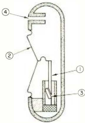
Figure 1. Sectional view of mechano-electronic transducer. (1) variable tube element, (2) paper diaphragm, (3) fixed element, (4) low frequency port.
