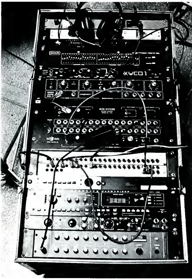
Suzanne Ciani's innovative "Voice Box," featuring the Polyfusion FF-1 Frequency Follower, Bode Model 7700 Vocoder, Eventide H949 Harmonizer® and Marshall Time Modulator.
