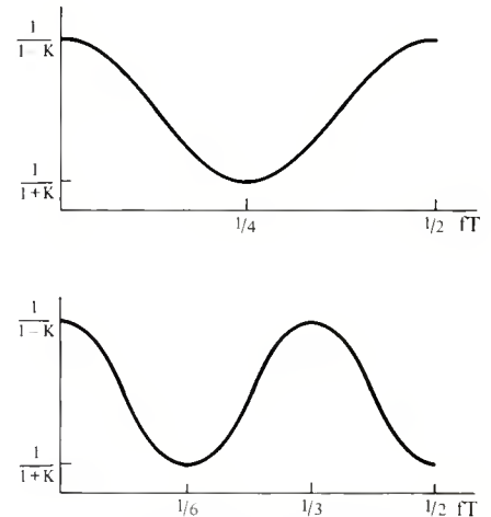
Figure 5. The frequency response of an IIR filter when the delay is (A) two sampling intervals long, and (B) three sampling intervals long.
