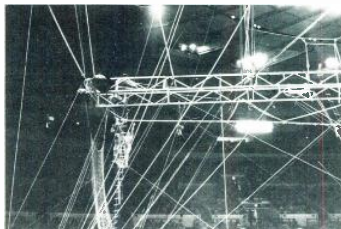
The loudspeaker array mounted at the end of the grid over Ring One.
