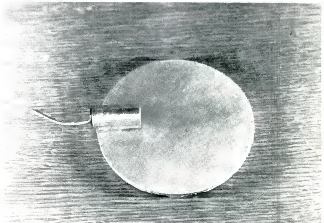
Figure 5. The ZAP attached to a 3 1/2-in. diameter circle of 1/8-in. aluminum.
