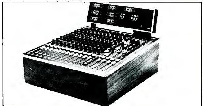
Figure 8. The MCI/Sony JH-800 Compact Console.
