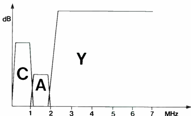
Figure 2. Comparison chart of video head frequency spectrum.
