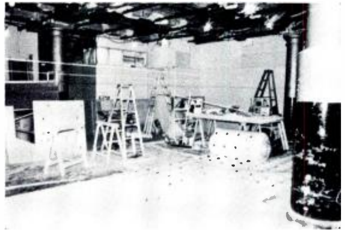
Flooring being laid—rubber isolators imbedded in fiberglass with a section of floor laid over it.
