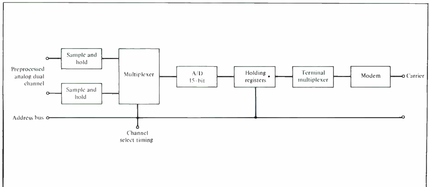
Figure 4. The ADDS system, showing a dual-channel analog program processed for digital transmission via satellite.
