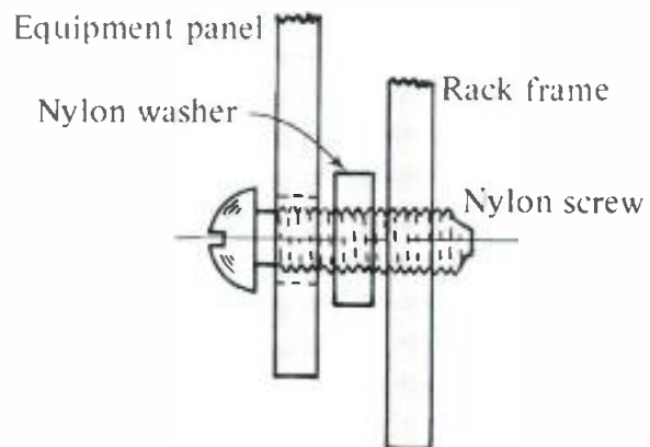
Figure 4. In the case of particularly hum-sensitive gear, nylon washers and screws may be used for better isolation.
