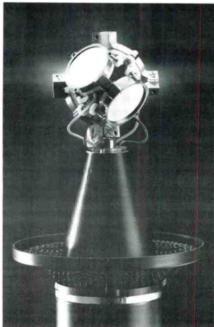
The Calrec Soundfield capsule.
