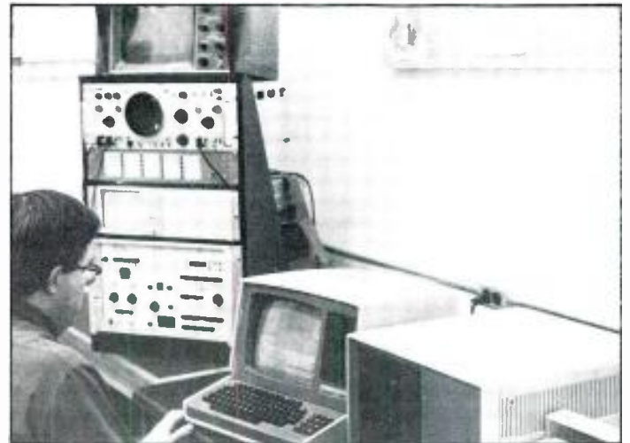
Figure 4. Outputs from the FFT system are compared to determine the difference between two microphones' frequency responses.
