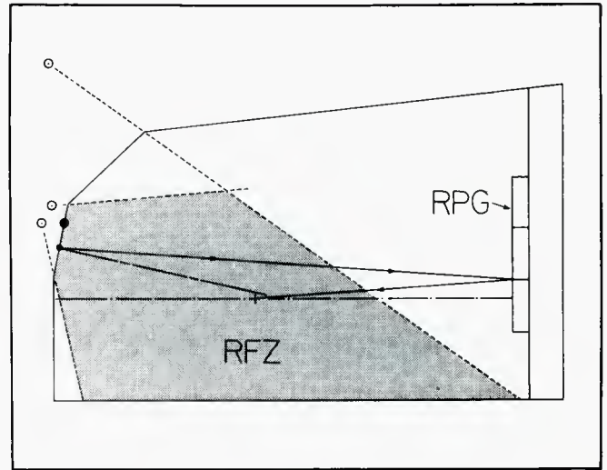
Figure 1B. Elevation for an RPG/RFG control room showing virtual sources (open circles) of woofer (large dot) from front wall, RFZ baffle and ceiling, which affect limiting RFZ reflections (dashed lines). Direction (solid line) of incident sound from the tweeter (small dot) and reflected sound from an RPG cluster is shown along with tweeter orientation (long-short dash).
