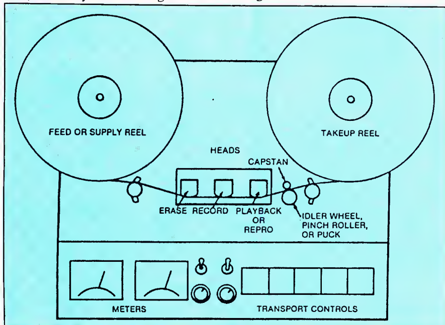
Figure 1. The major parts of a typical tape recorder.
