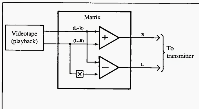
Figure 6. A means for decoding the pre-recorded Carson shows before sending them to the transmitter.
