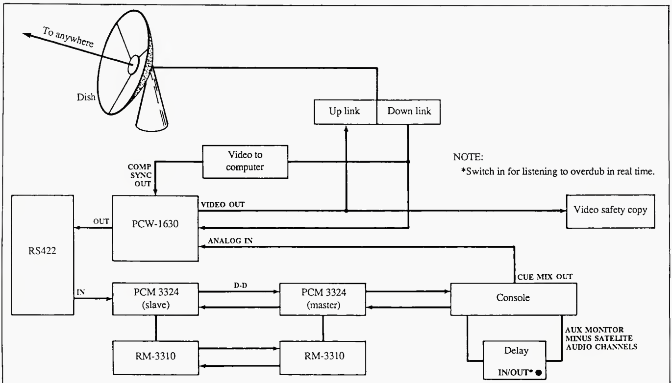
Figure 1. The basic flow chart of the entire satellite, audio, and video systems
