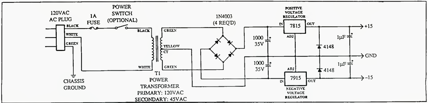
Figure 2. The power supply schematic
