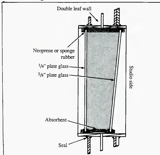
Figure 3. The cross section of the control room wall containing the double-glass window. Note the skewing of the studio side glass
