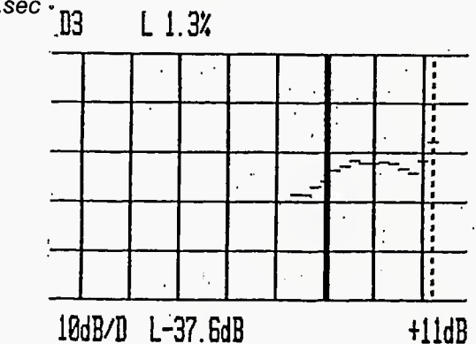
Figure 5B. Third order distortion vs. record level at 15 in.sec
