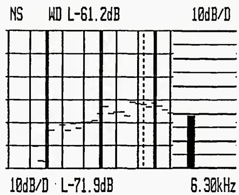
Figure 4B. S/n at 7.5 in/sec A-weighted
