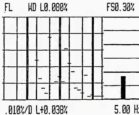
Figure 8B. Wow and flutter analysis at 7.5 in/sec weighted
