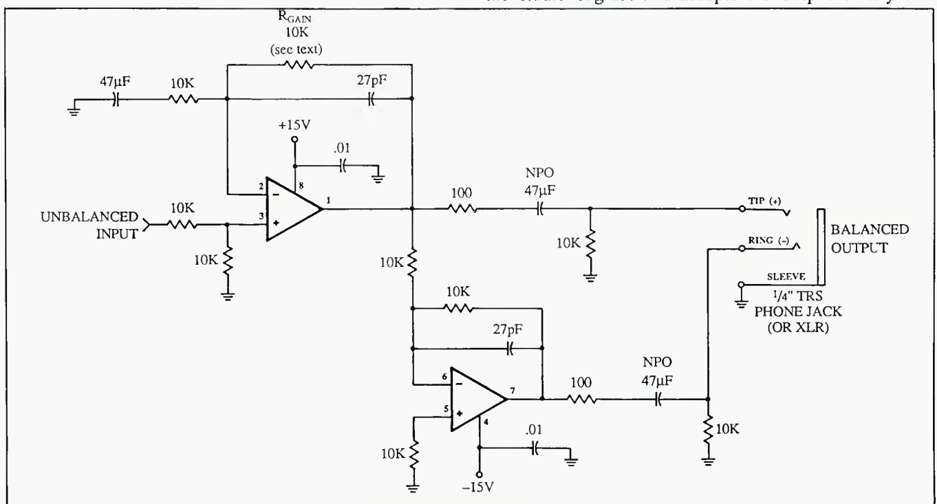
Figure 1. Schematics for OA-1 Balanced Output Interface and associated Power Supply
