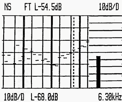
Figure 3A. S/n analysis at 15 in./sec unweighted
