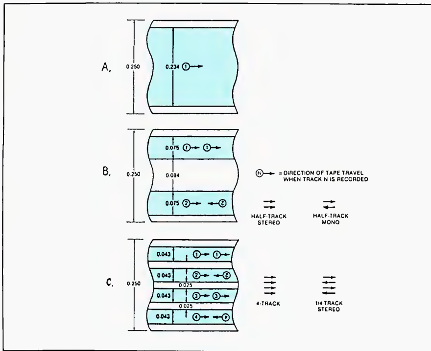
Figure 3. Some track-width standards for quarter-inch tape
