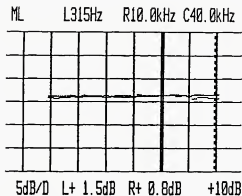
Figure 9A. Maximum output level (linearity) at 315 Hz and 10 kHz at 15 in/sec
