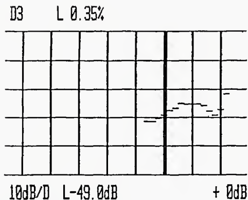
Figure 6A. Third order distortion vs. record level at 7.5 in/sec
