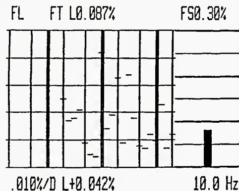
Figure 7A. Wow and flutter analysis at 15 in/sec unweighted
