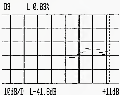
Figure 6B. Third order distortion vs. record level at 7.5 in/sec
