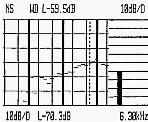
Figure 3B. S/n analysis at 15 in/sec A-weighted
