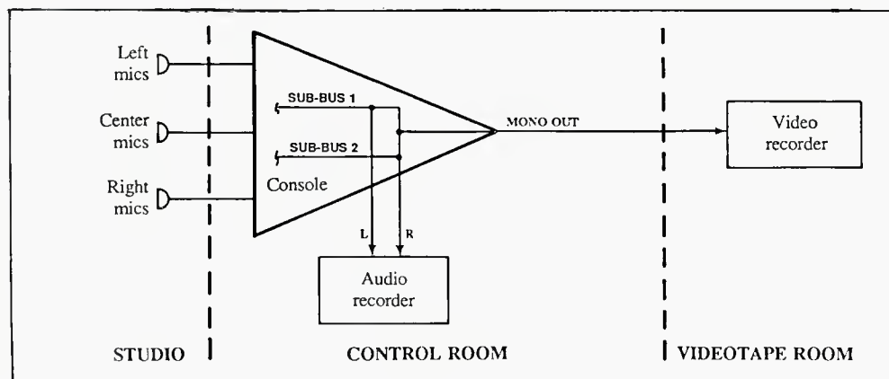
Figure 4. An early method of recording the show in stereo on audio tape, and in mono on videotape.
