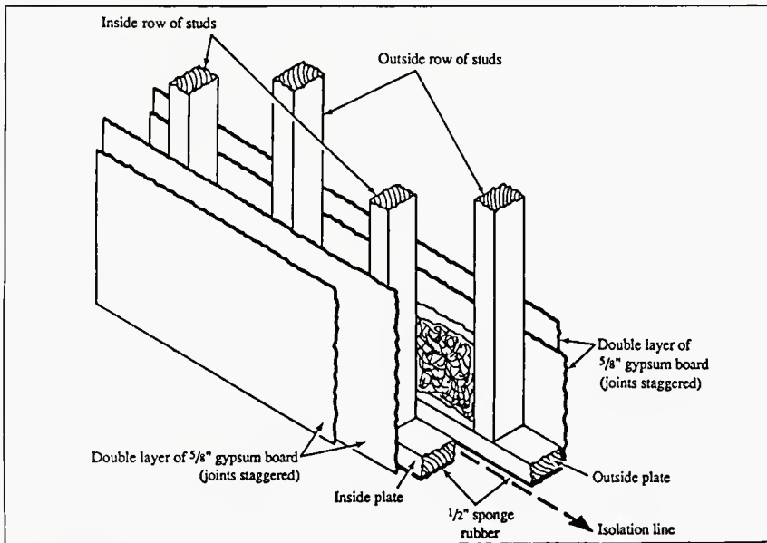
Figure 2. Cross section and composition of wall separating the control room from the main studio
