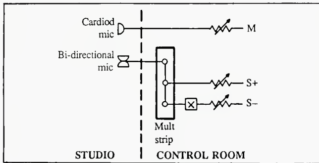
Figure 9. The setup for "coincident" or M/S mic-ing occasionally used by Estes as a point-source pickup for solo performers.
