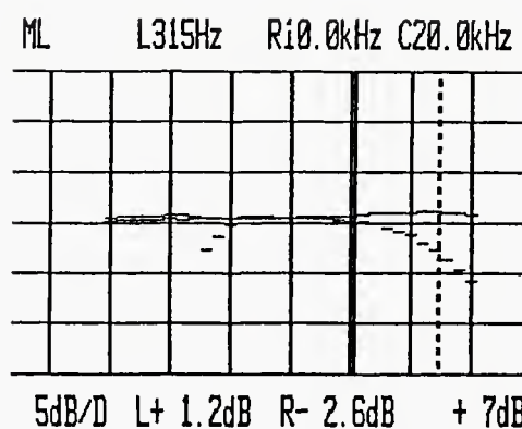
Figure 9B. Maximum output level (linearity) at 315 Hz and 10 kHz at 7.5 in/sec
