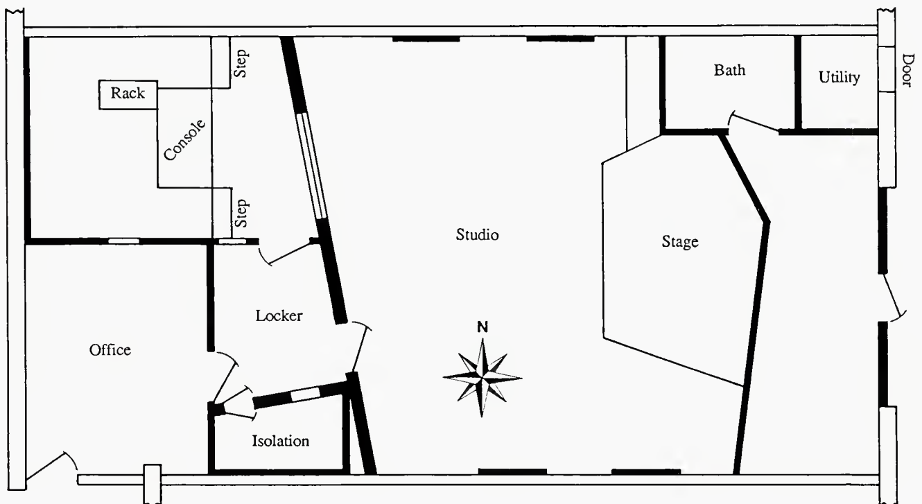
Figure 1. Dragonville Studios floor plan
