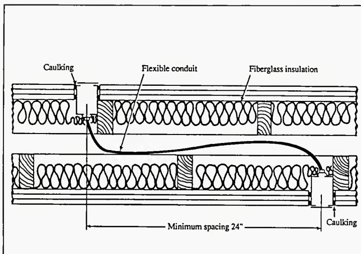
Figure 4. The cross section of the studio/control room wall. Note the staggered access openings
