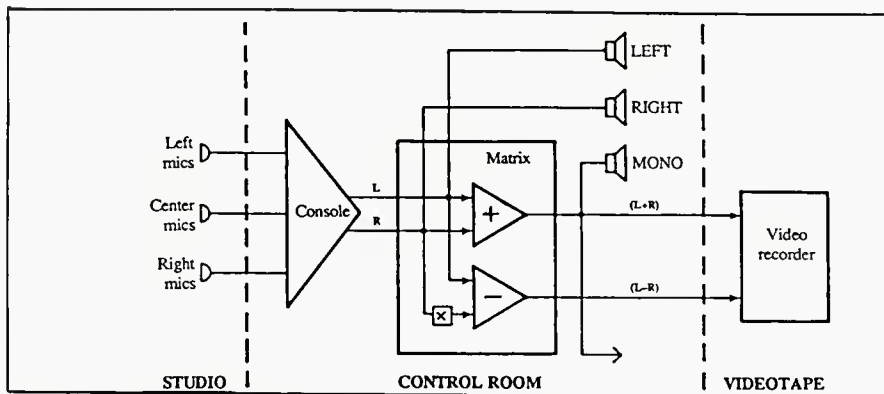
Figure 5. The setup Estes used temporarily to record both mono and stereo on video tape using only two console outputs.
