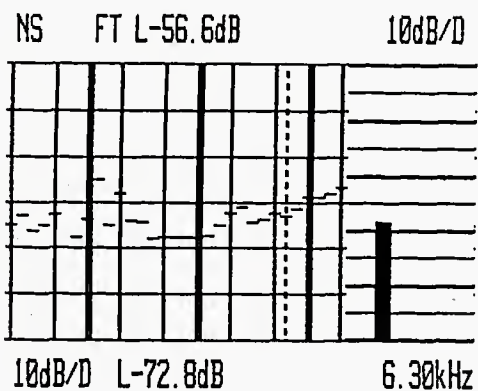
Figure 4A. S/n at 7.5 in./sec unweighted
