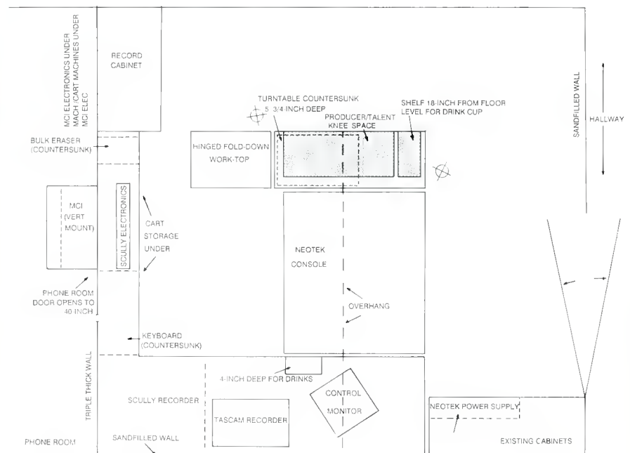
Figure 2. The new audio booth design at KSLA-TV.
