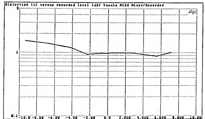
Distortion versus recorded level, Yamaha MT2X, at 9.5 cm. per second, with dbx ON
