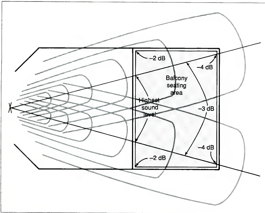
Figure 7. Overall coverage in the balcony from two horns.
