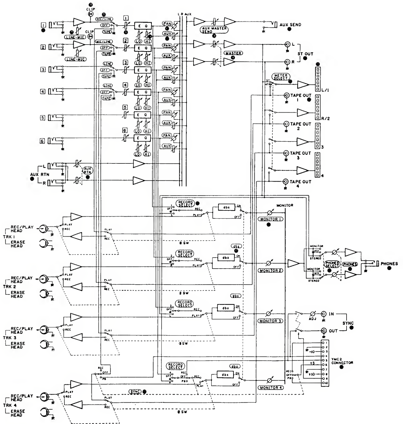
Figure 1. The block diagram.
