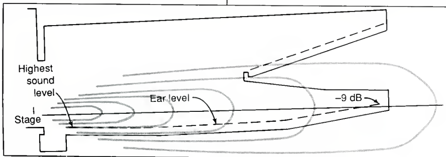
Figure 3. Improved coverage from a better choice of horn type.
