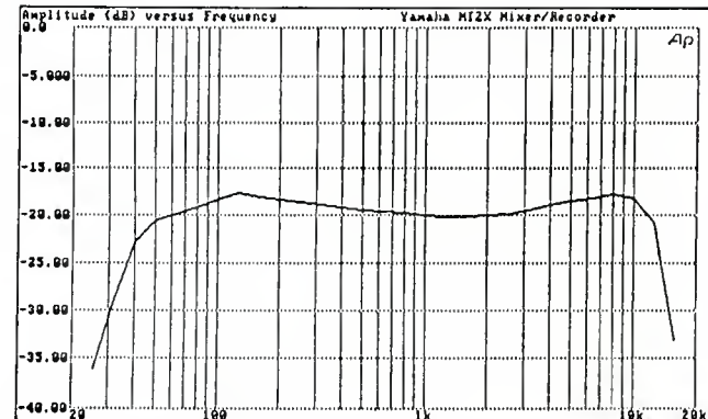
Frequency Response, record/play at 4.8 cm/sec, -20 dB record level, dbx ON, Yamaha MT2X Multitrack Cassette Recorder
