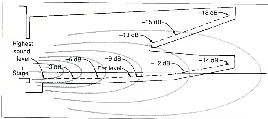
Figure 2. An overlay showing vertical dispersion for a typical horn application.
