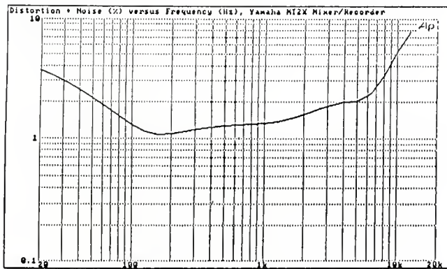
Distortion vs Frequency Yamaha MT2X Multitrack Cassette Recorder, at 4.8 cm/sec
