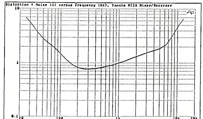
Distortion vs Frequency Yamaha MT2X Multitrack Cassette Recorder, at 4.8 cm/sec, dbx ON
