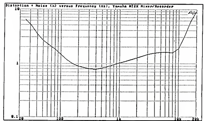
Distortion vs Frequency Yamaha MT2X Multitrack Cassette Recorder, at 9.5 cm/sec, dbx ON.
