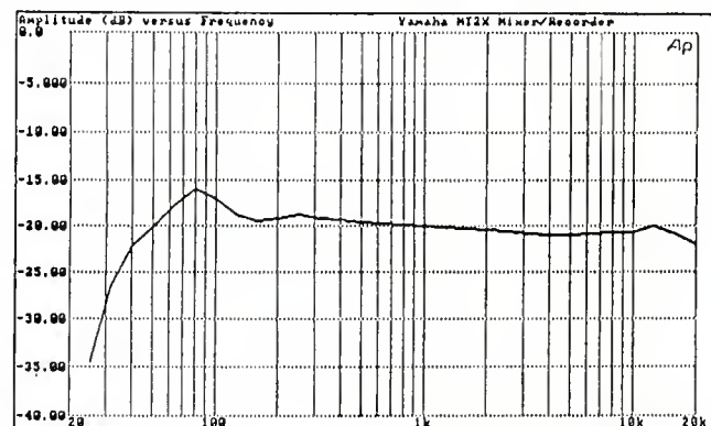
Frequency Response, record/play at 9.5 cm/sec, -20 dB record level, dbx ON, Yamaha MT2X Multitrack Cassette Recorder
