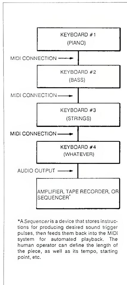
Figure 1. A schematic of a possible MIDI configuration.
