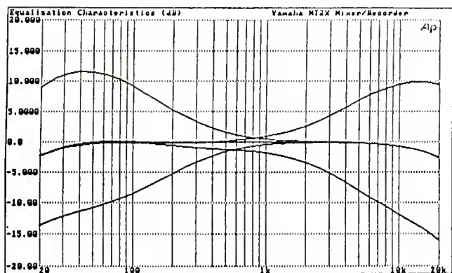
Equalization characteristics, Yamaha MT2X Multitrack Cassette Recorder, (controls set for maximum boost and cut)
