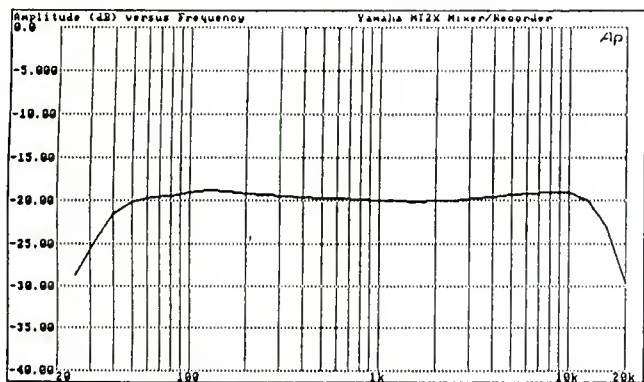
Frequency Response, record/play at 4.8 cm/sec, -20 dB record level, Yamaha MT2X Multitrack Cassette Recorder
