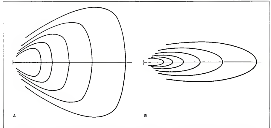
Figure 1. Dispersion overlays for a 90° x 40° horn. (A) horizontal, (B) vertical.
