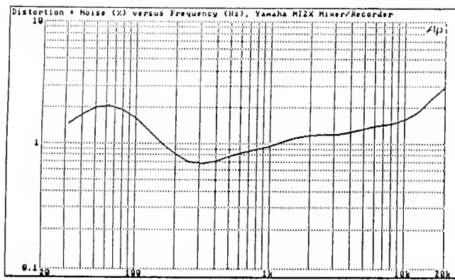
Distortion vs Frequency Yamaha MT2X Multitrack Cassette Recorder, at 9.5 cm/sec
