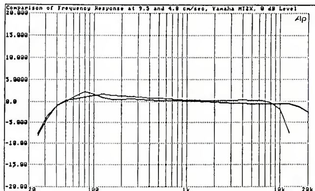
Record play frequency response, at 0 dB level, Yamaha MT2X. Earlier roll-off occurs at slower (4.8 cm/sec.) speed.
