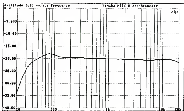
Frequency Response, record/play at 9.5 cm/sec, -20 dB record level, Yamaha MT2X Multitrack Cassette Recorder
