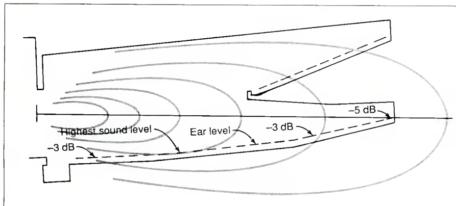
Figure 4. Still better coverage from a better horn location.
