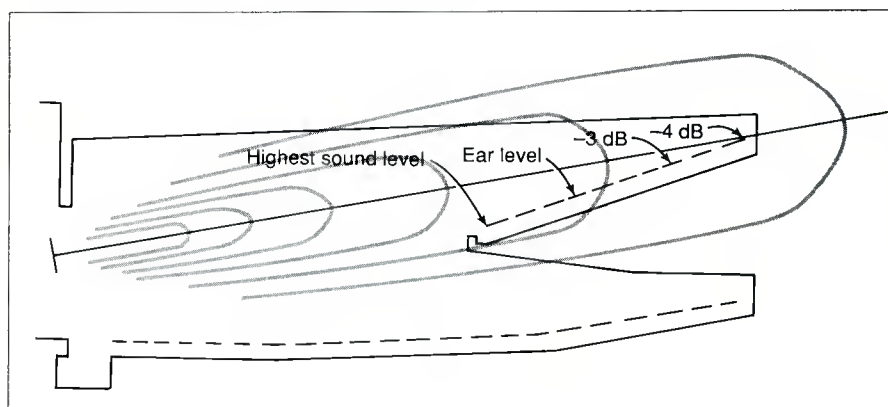
Figure 6. Vertical coverage in the balcony.
