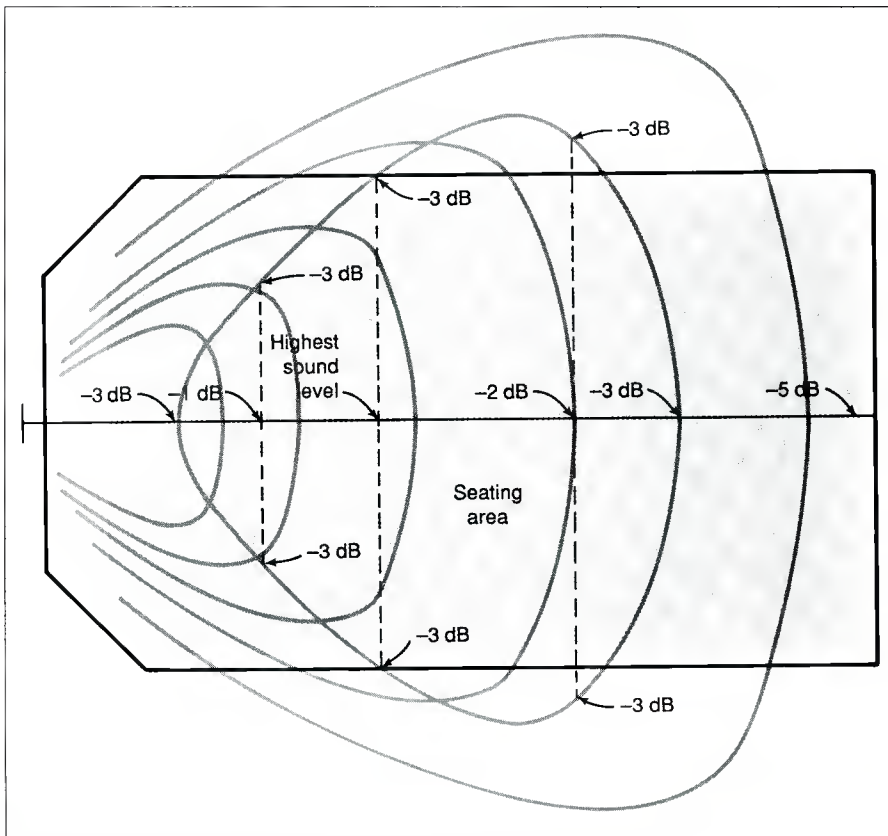
Figure 5. Horizontal dispersion and overall coverage contour.
