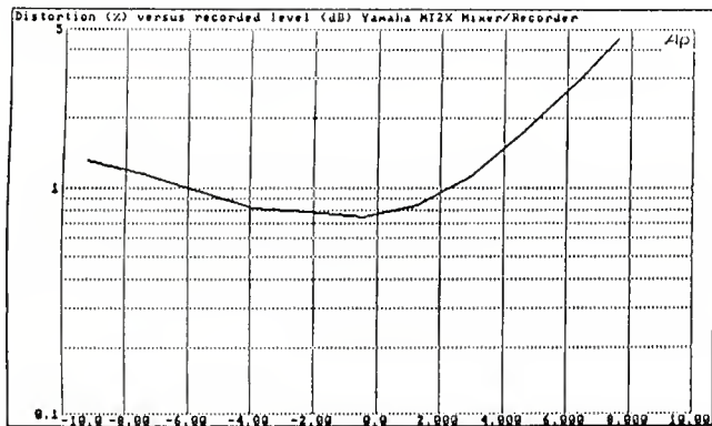
Distortion versus recorded level, Yamaha MT2X, at 9.5 cm. per second.
