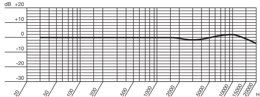
Cardioid On-axis Frequency Response (measured at 1 meter)
