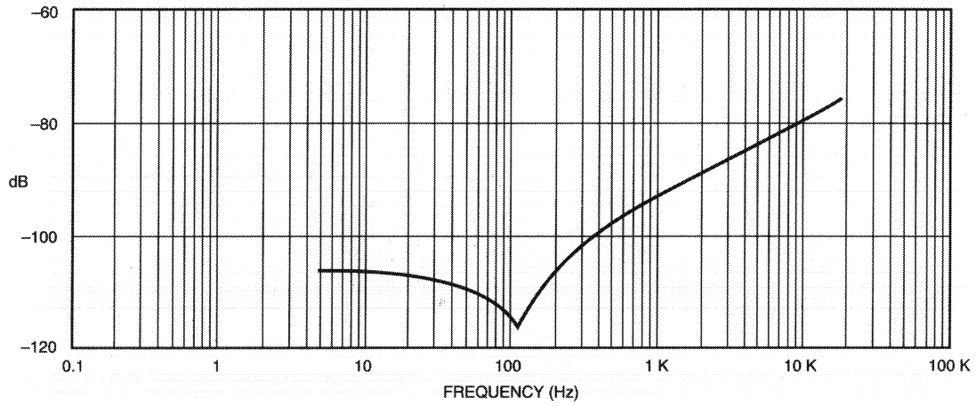
Fig. 7.6 Nominal Crosstalk (75 watts into 8 ohms with one channel driven)
