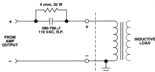
Fig. 3.7 Connection to an Inductive Load
