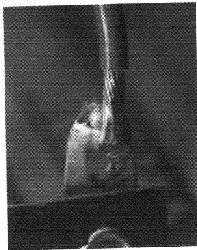
Fig. 7.7 Disturbed Joint
