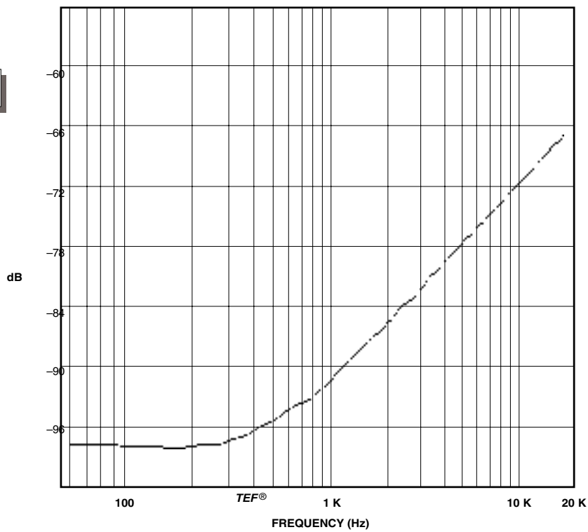
Fig. 6.7 Typical Crosstalk
