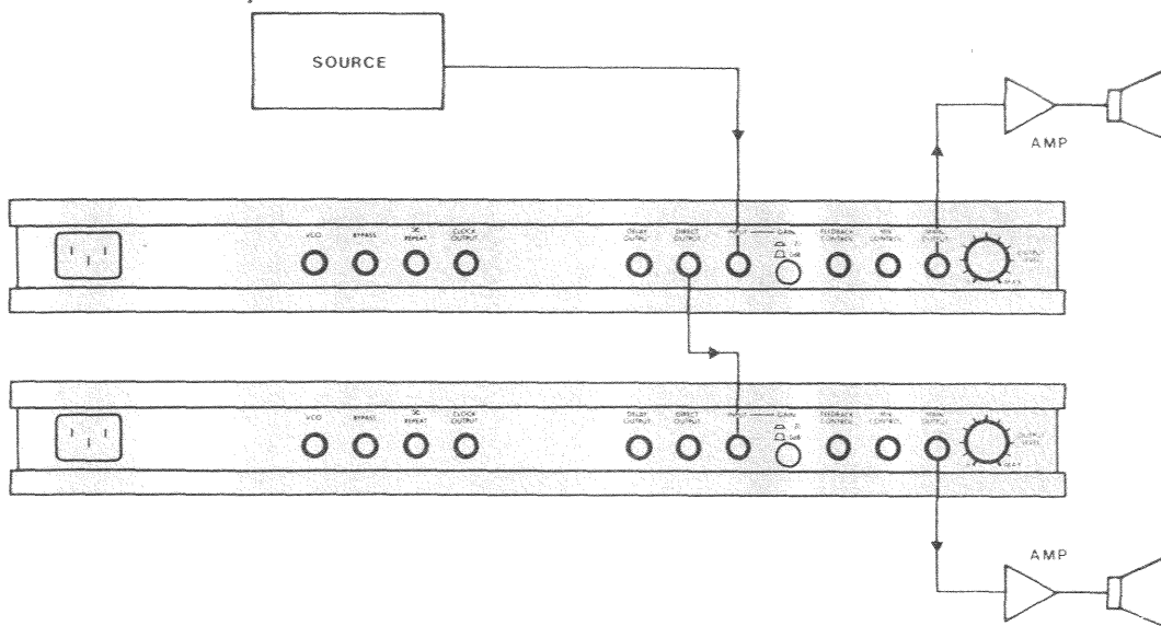
Figure 4.8 — PARALLEL CONNECTION OF TWO PCM 42s
