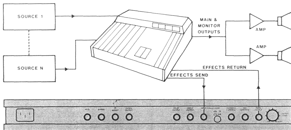
Figure 4.4 – BASIC RECORDING OR SOUND REINFORCEMENT SETUP
