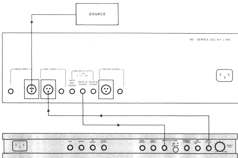
Figure 4.9 — CONNECTION OF PCM 42 WITH LEXICON 90-SERIES DELAY LINES
