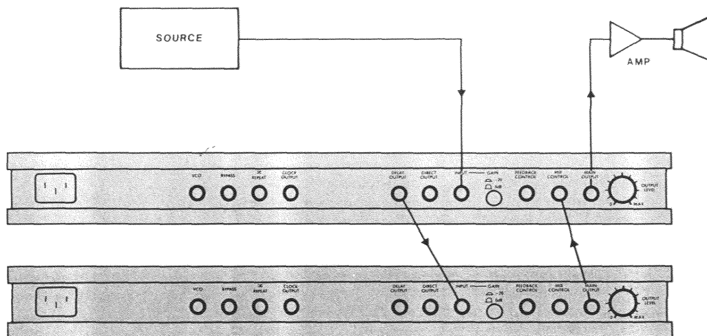
Figure 4.7 – SERIES CONNECTION OF TWO PCM 42s
