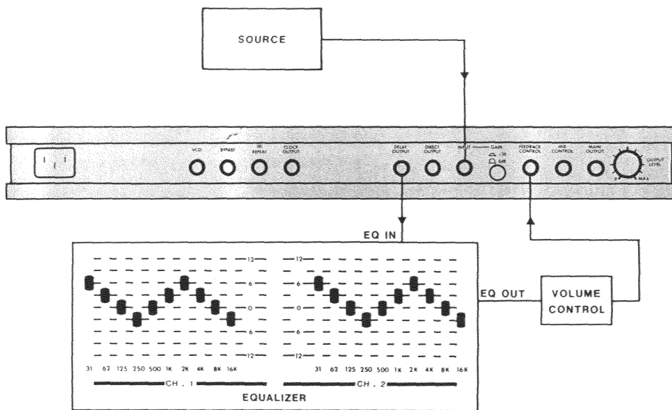
Figure 4.11 — CONNECTION OF PCM 42 WITH EQUALIZED FEEDBACK
