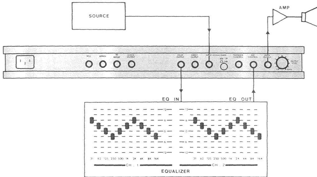
Figure 4.10 — CONNECTION OF PCM 42 WITH EQUALIZED OUTPUT
