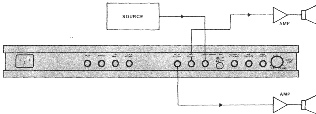
Figure 4.12 — SOUND REINFORCEMENT WITH ONE REMOTE ZONE OF SPEAKERS
