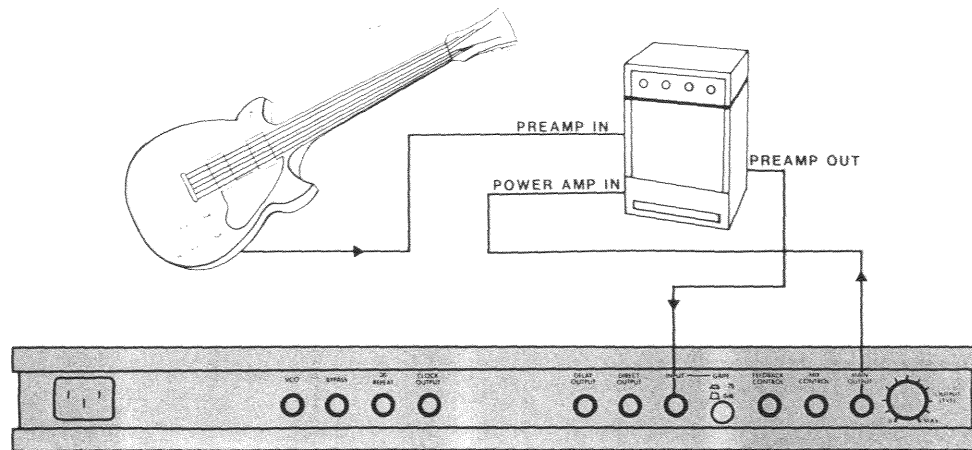
Figure 4.2 — BASIC SETUP WITH AMPLIFIER EFFECTS LOOP
