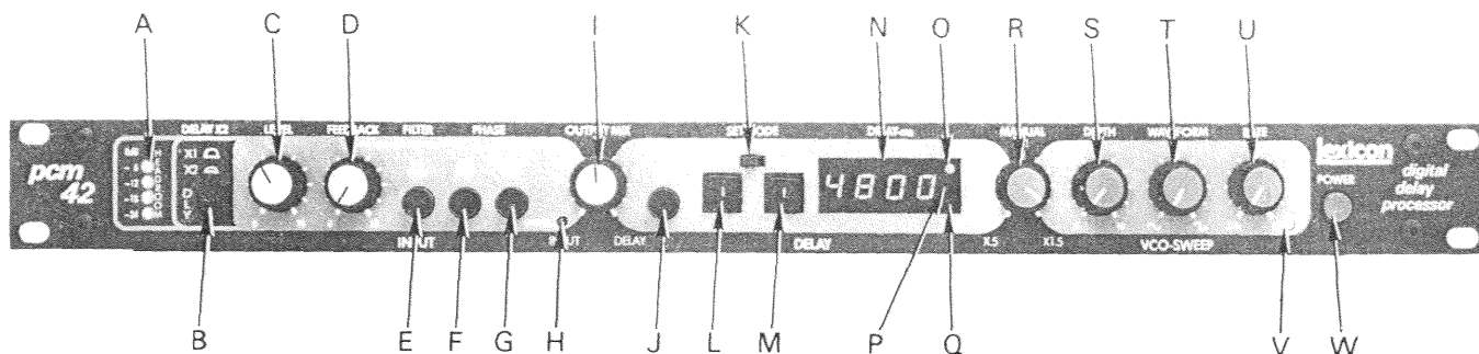
Figure 2.1 — PCM 42 Front Panel
