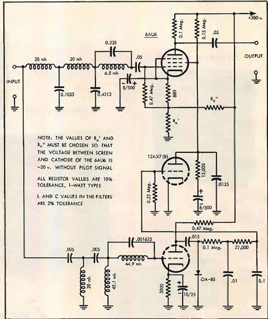
Fig. 3. Schematic diagram of electronic switch with filters and rectifier.
